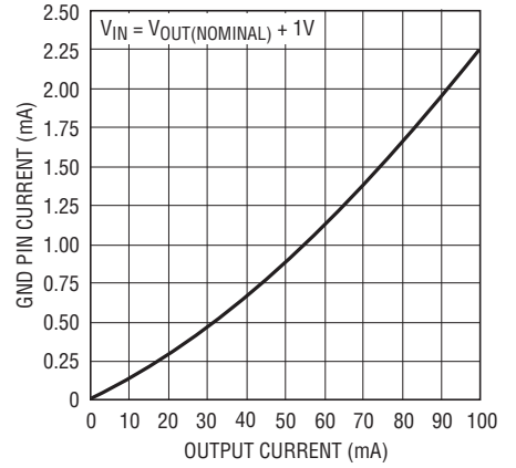
Output 2 GND Pin Current vs I_{LOAD}
