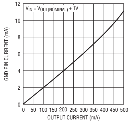
Output 1 GND Pin Current vs I_{LOAD}
