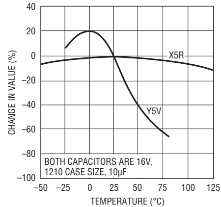
Figure 5. Ceramic Capacitor Temperature Characteristics
