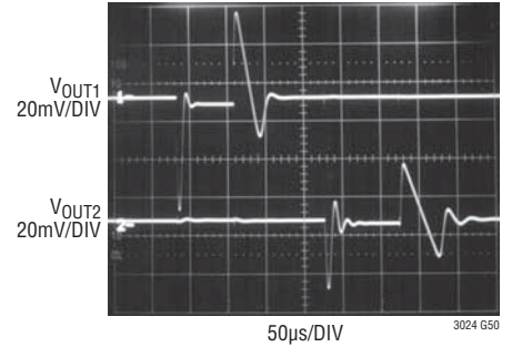
Channel-to-Channel Isolation
